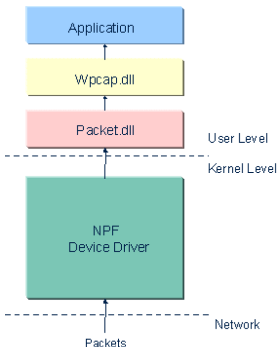
Figure 28: WinPcap Architecture
