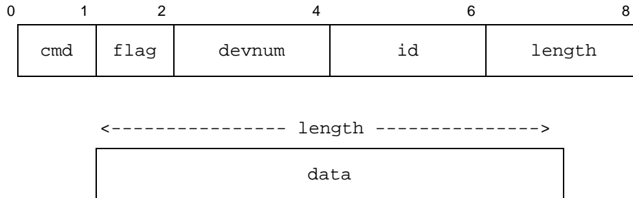
Figure 18: Shared Device Server – Client Header Structure
