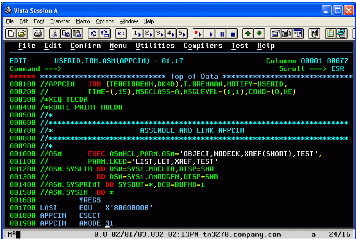
Figure 34: Vista tn3270 Window
