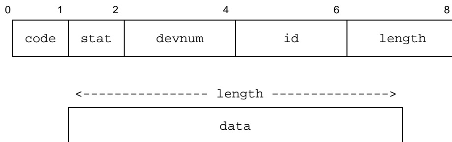
Figure 19: Shared Device Server – Server Header Structure
