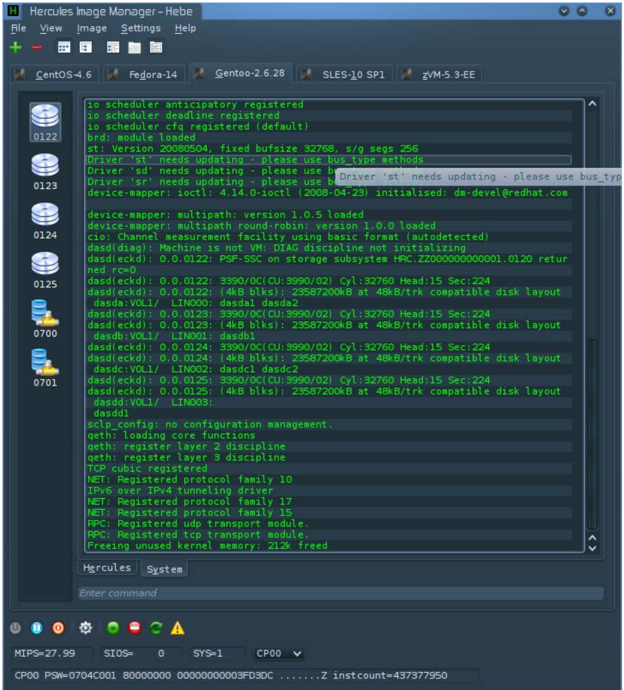
Figure 23: Hebe (system console)
