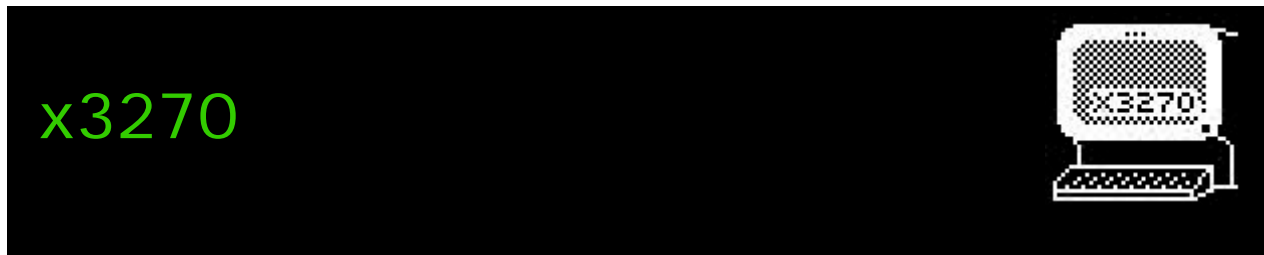
Figure 35: x3270 Logo
