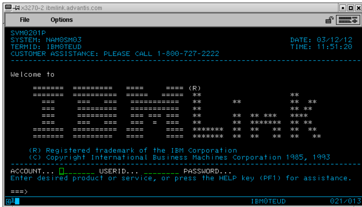
Figure 36: x3270 Window
