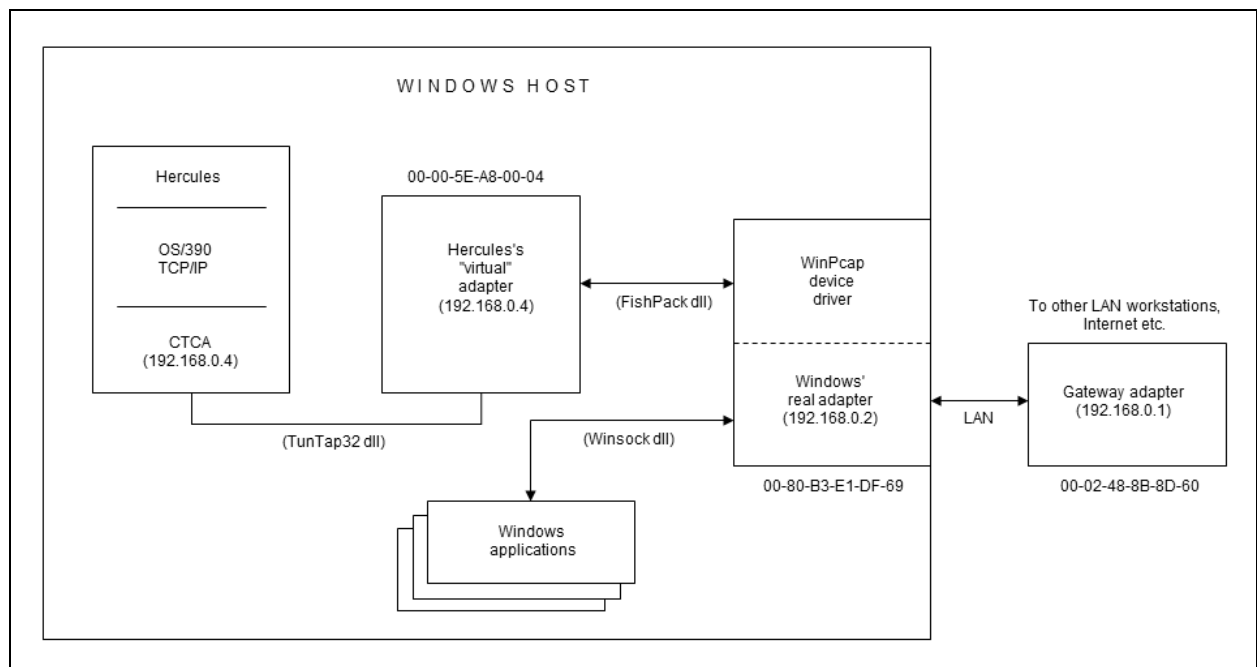
Figure 32: CTCI-WIN Implementation
