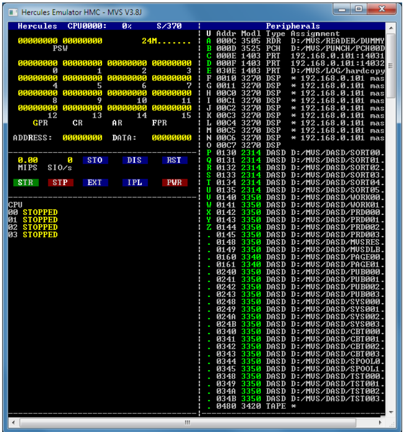
Figure 1: Hercules Hardware Console – Device and status window
