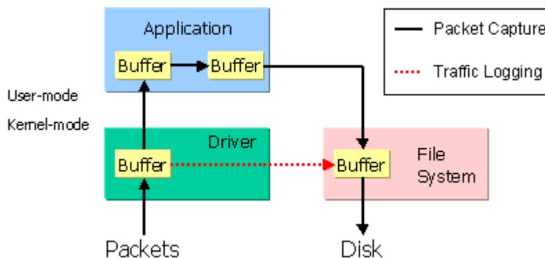
Figure 31: Packet Capture vs. Kernel-Level Dump
