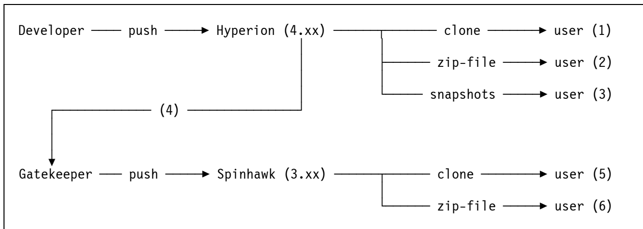
Figure 4: Hercules Repository Structure
