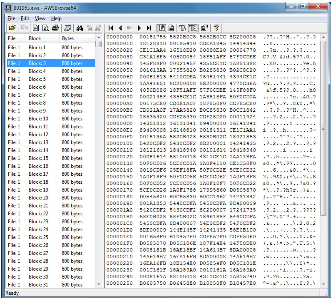
Figure 40: AWS Browse Main Window
