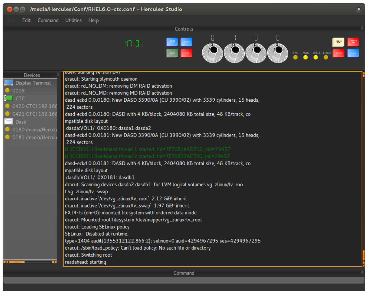
Figure 21: Hercules Studio Main Panel
